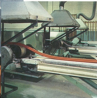
Multiple extrusion lines
